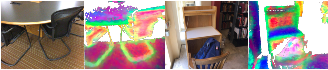
Fig. 3: Generalizable NeRFs acquire geometric and semantic priors: RGB images are input views from ScanNet [8], color images are PCA visualizations of feature volume projected to the input camera view encoded by an RGB-D Gen-NeRF [10] encoder. Note how semantically similar structures acquire similar features.
