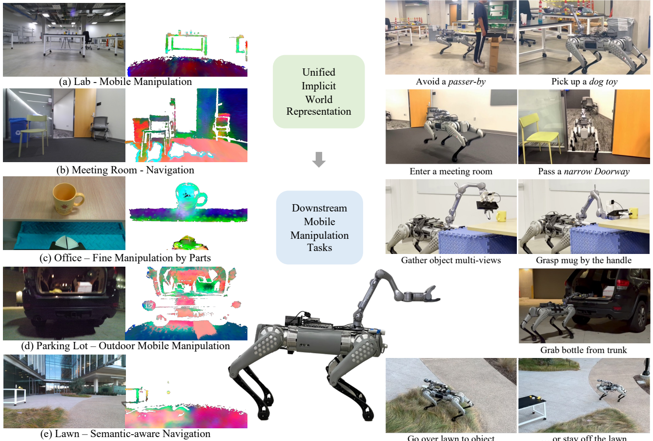
Fig. 1: GeFF , Generalizable Feature Fields , provide unified implicit scene representations for both robot navigation and manipulation in real-time. We demonstrate the efficacy of GeFF on open-world mobile manipulation , semantic-aware navigation , and zero-shot manipulation by parts under diverse scenes ((a) work in a lab where a person walks in, (b) enter a meeting room with narrow entrance, (c) fine part-level manipulation, (d) grasp objects in a parking lot, and (e) semantic-aware navigation near a lawn). The visualization of the feature fields is obtained by PCA of rendered features. For best illustration, please check out the supplementary video.
