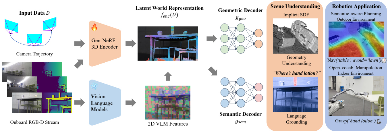
Fig. 2: Pre-trained as a generalizable NeRF encoder, GeFF provides a unified scene representation to support robot tasks from an onboard RGB-D stream, offering both real-time geometric information for planning and language-grounded semantics query capability. Compared to LERF [20], GeFF runs in real-time without costly per-scene optimization, which enables many potential robotics applications. We demonstrate the efficacy of GeFF in open-world language-conditioned mobile manipulation . Feature visualizations are done by running PCA on high-dimensional feature vectors and normalizing the 3 main components as RGB.
